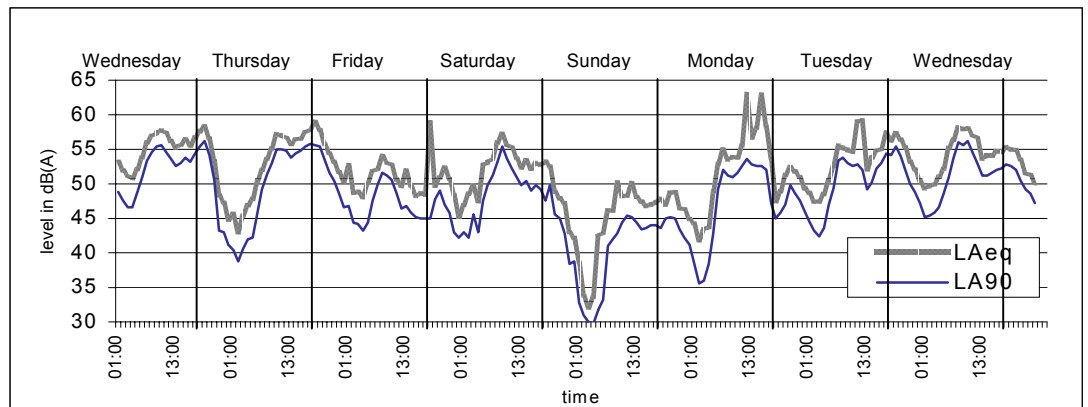
Figure 1.9 — Eight days of hourly L_{A90,1h} and L_{Aeq,1h} readings
