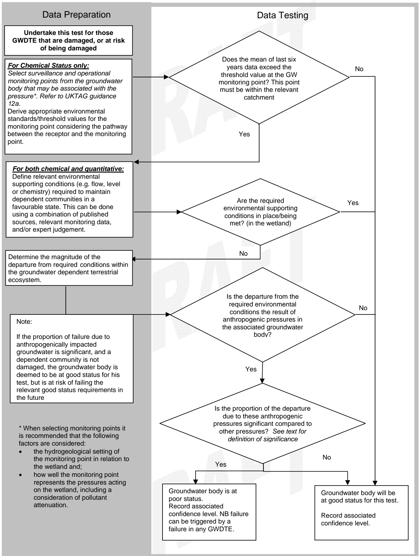
Figure 2 : Outline of procedure and data preparation for status test for significant damage to groundwater dependent terrestrial ecosystems
